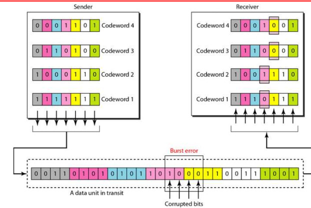
Figure 10.13 Burst error correction using Hamming code
