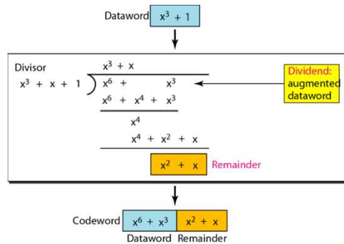
Figure 10.22 CRC division using polynomials
