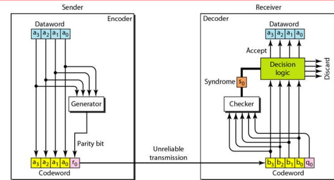
Figure 10.10 Encoder and decoder for simple parity-check code
