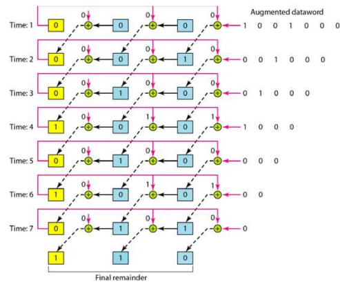
Figure 10.18 Simulation of division in CRC encoder
