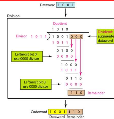
Figure 10.15 Division in CRC encoder
