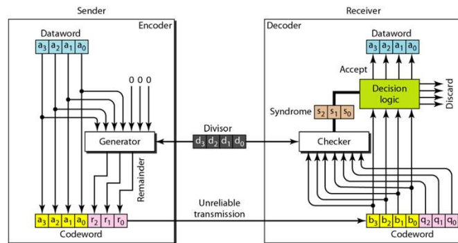
Figure 10.14 CRC encoder and decoder
